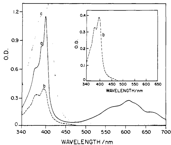
Figure 1. Absorption spectra of disproportionation products of C_8V^{2+} : (a) Composite spectrum of C_8V^+ and C_8V in ethyl acetate; (b) spectrum of C_8V in ethyl acetate, after subtraction of the C_8V^+ spectrum; (c) spectrum in toluene.
